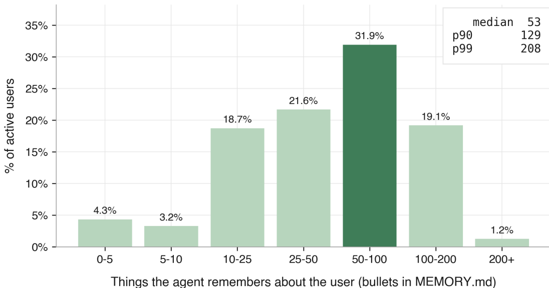
Figure 7. Distribution of “things I remember about you” across the active Portal user base. Each item is one bullet in the user’s MEMORY.md — a fact, a preference, or a lesson the agent has committed to long-term storage. The number is exposed to every user on portal.ai/me .
