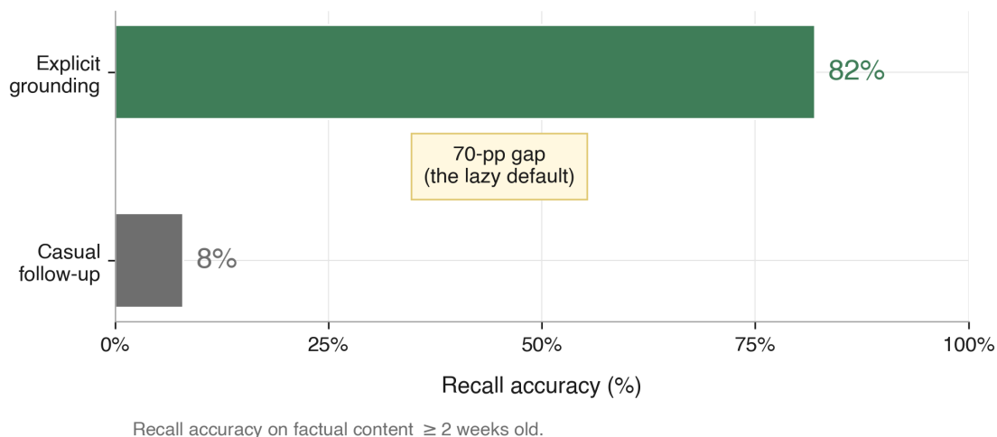
Figure 5. Recall accuracy on factual questions about user content from 2+ weeks earlier, under two prompting conditions. The pre-reply gate (Layer 2) eliminates the gap structurally — every interactive turn runs the gate; retrieval becomes a guarantee.
